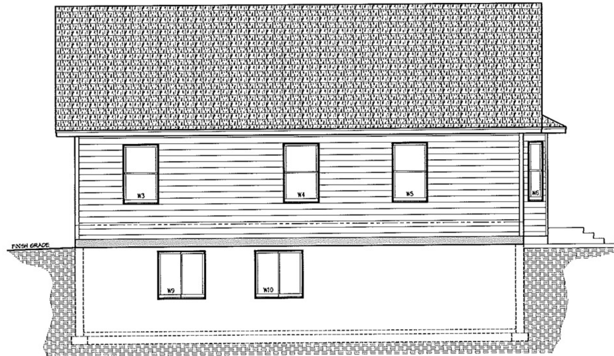
REAR EXTERIOR ELEVATION
