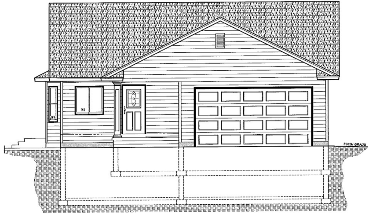
FRONT EXTERIOR ELEVATION
